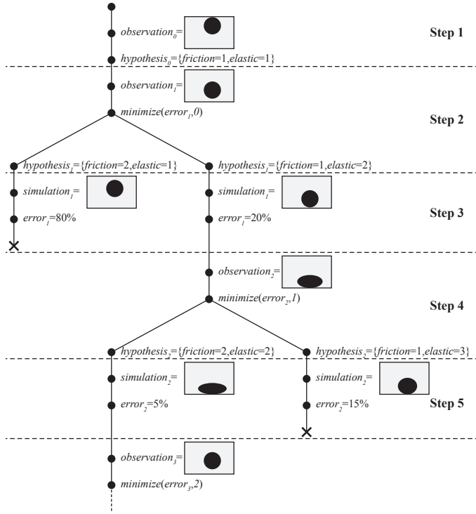
Figure 5: An example of learning in a tableau
